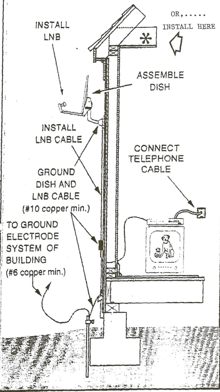
TYPICAL INSTALLATION
